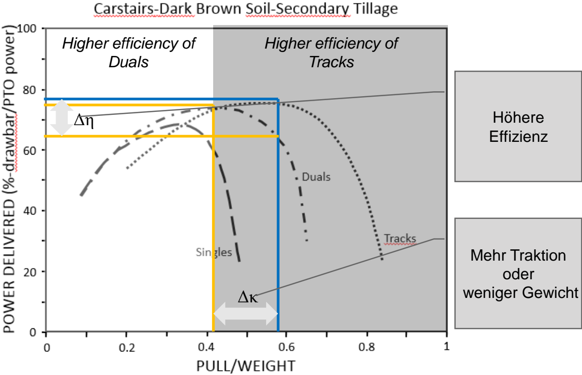
Power Delivery Efficiency vs. Pull to Weight at 16400 kg total tractor weight
